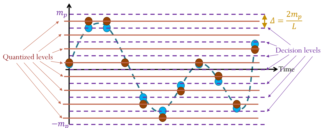
Figure 74: Quantized levels
