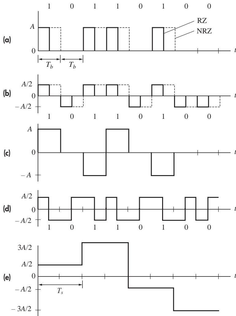
Figure 76: Line codes with rectangular pulses: (a) unipolar RZ and NRZ; (b) polar RZ and NRZ; (c) bipolar NRZ; (d) split-phase Manchester; (e) polar quaternary NRZ. [3, Fig 11.1-1 p 483]
